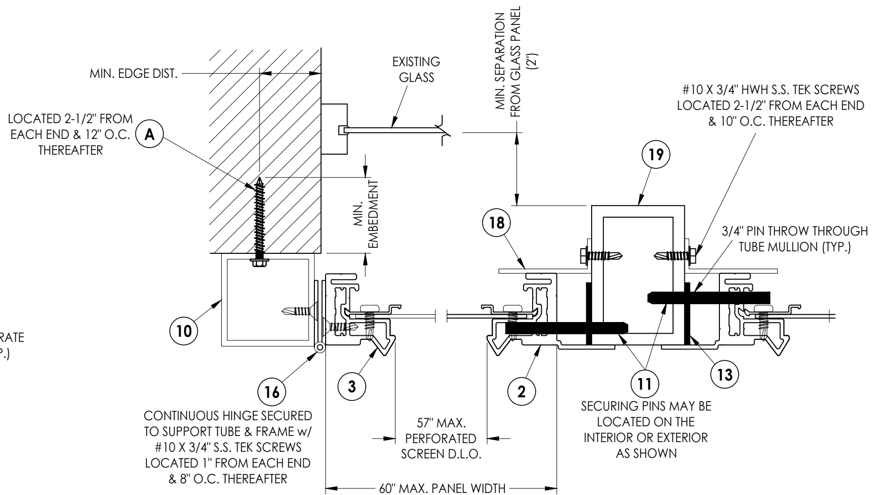
2 HORIZONTAL CROSS SECTION 4 FACE MOUNT
