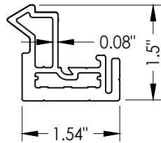
3 ENHANCED SUBFRAME
