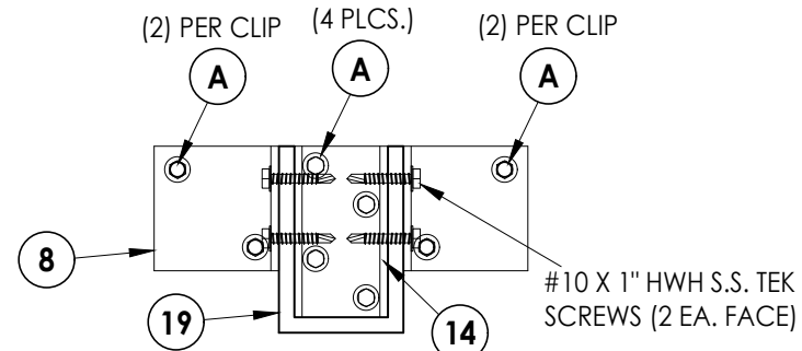
SECTION C-C INSET MOUNT
