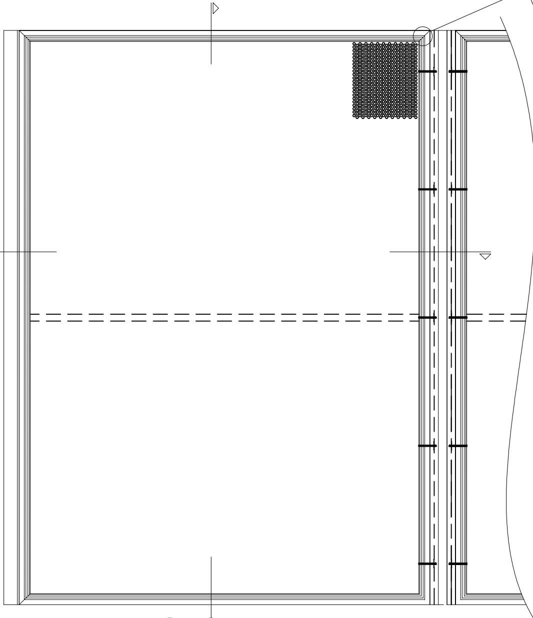
SUBFRAME CORNER DETAIL
