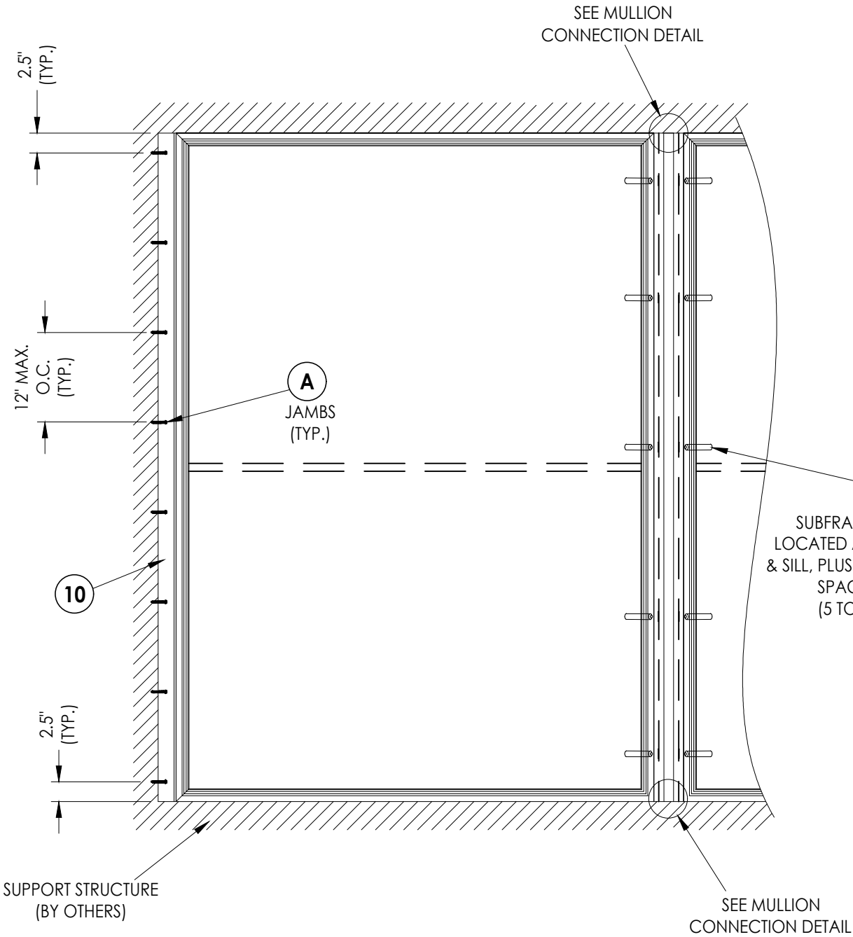
INSET MOUNT FRAME ANCHORING
