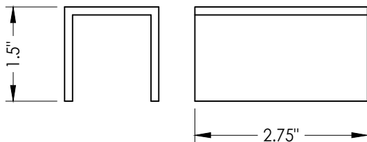
14 TUBE MOUNTING CHANNEL 0.125" THICK
