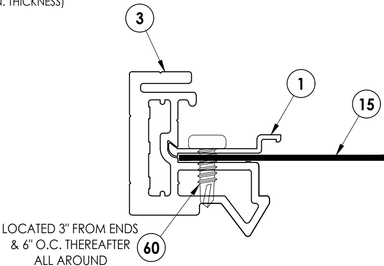
SCREEN INFILL ATTACHMENT DETAIL
