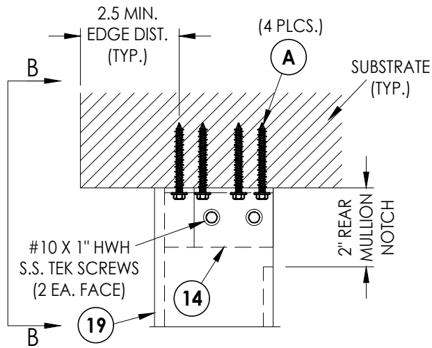
SECTION THROUGH MULLION INSET MOUNT
