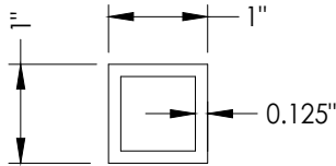
7 MID-HEIGHT SUPPORT TUBE
