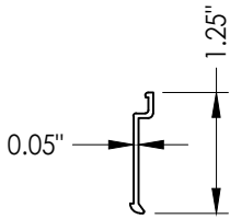
1 BARRIER RAIL
