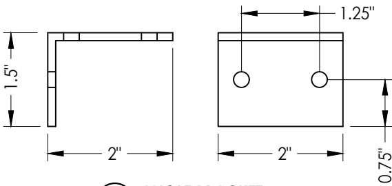
8 ANGLE BRACKET 0.125" THICK
