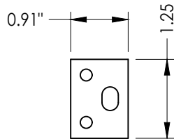
13 PIN REINFORCEMENT/LOCATOR 0.079" THICK
