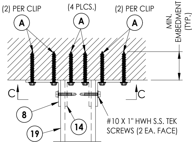
SECTION C-C INSET MOUNT
