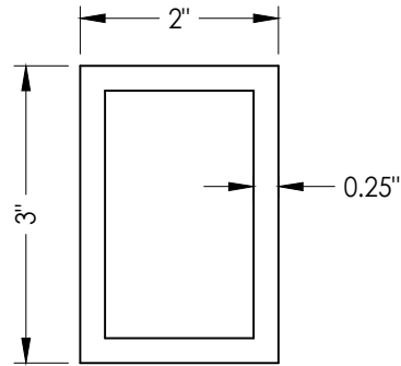
19 TUBE MULLION
