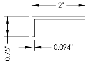
18 STOP ANGLE
